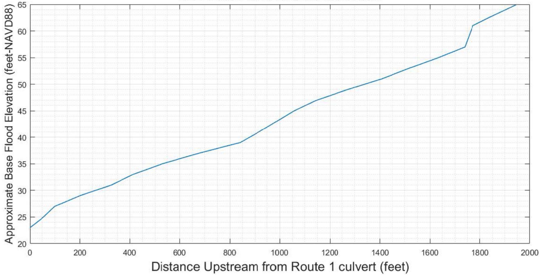
Base Flood Profile for Unnamed Stream
